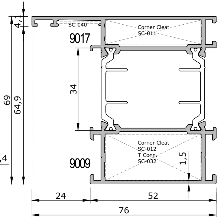
69-9009/9017 | 52 mm Kasa Profili 1.600 kg/m | 52 mm Frame Profile J_x=27,07 \text{ cm}^4 | J_y=18,46 \text{ cm}^4
