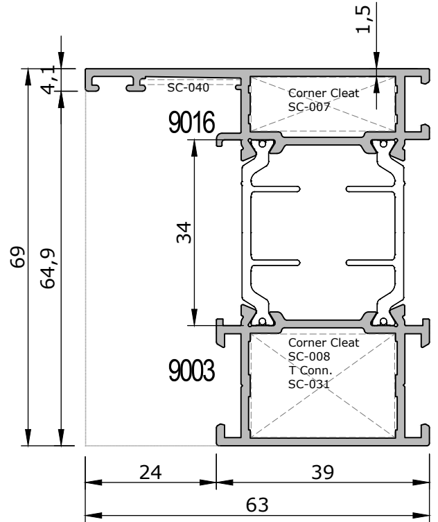
69-9003/9016 | 39 mm Kasa Profili 1.400 kg/m | 39 mm Frame Profile J_x=22,59 \text{ cm}^4 | J_y=9,75 \text{ cm}^4
