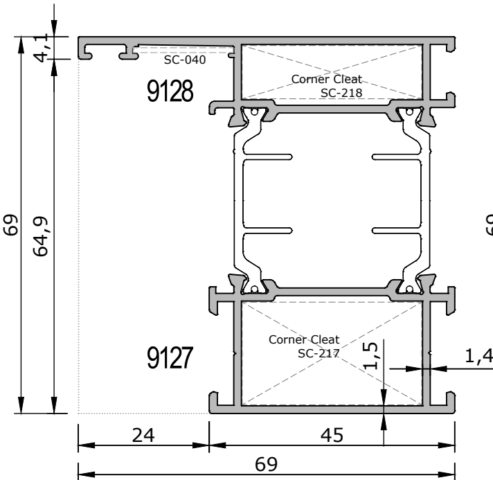
55-9127/9128 | 45 mm Kasa Profili 1.470 kg/m | 45 mm Frame Profile J_x=24,17 \text{ cm}^4 | J_y=13,14 \text{ cm}^4
