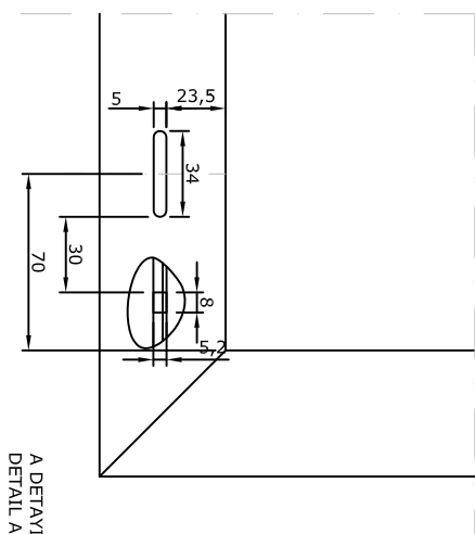
SABİT KASA SU TAHLİYE VE HAVALANDIRMA SEMASI FIXED FRAMES WATER DRAINAGE AND VENTILATION SYSTEM
