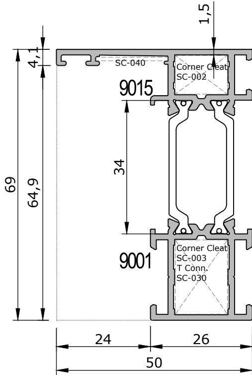
69-9001/9015 | 26 mm Kasa Profili 1.170 kg/m | 26 mm Frame Profile J_x=18,39 \text{ cm}^4 | J_y=4,24 \text{ cm}^4
